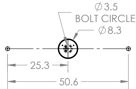
Mounting Detail MOUNTS TO J-BOX
