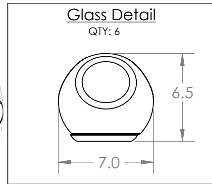
Mounting Detail MOUNTS TO J-BOX
