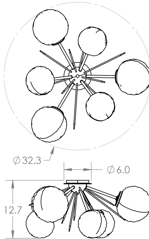
MINIMUM SIZE OF J-BOX REQUIRED IS 4" L x 4" W x 1.5" H
