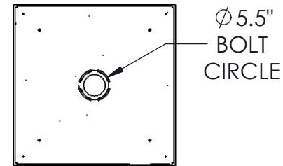
Mounting Detail MOUNTS TO STRUCTURE
