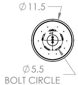
Mounting Detail Mounts Directly to Building Structure
