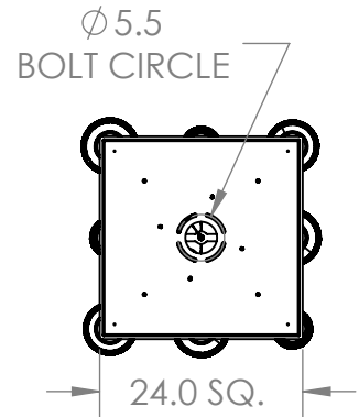
Mounting Detail Mounts Directly to Building Structure
