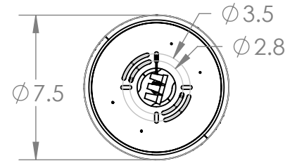
Mounting Detail Mounts to Ceiling J-Box
