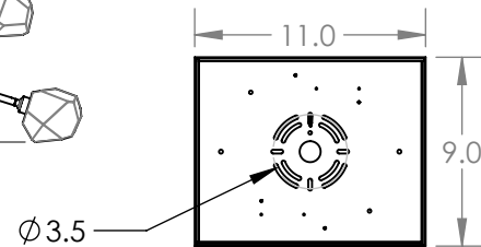
Mounting Detail Mounts to Building Structure
