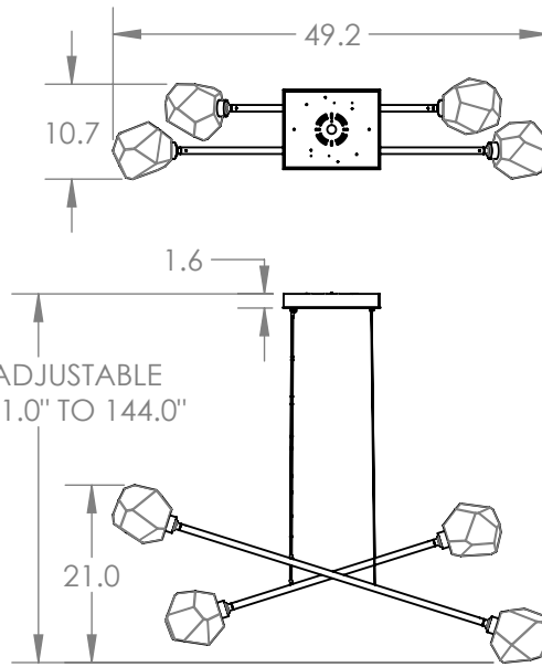
Mounting Detail Mounts to Building Structure
