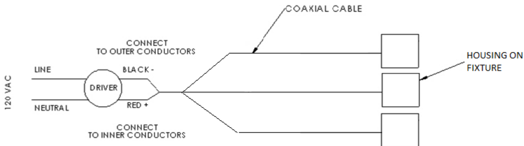
CONNECT THREE HOUSINGS TO ONE DRIVER
